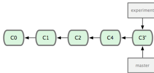
Figure 3.30: Fast-forwarding the master branch.
