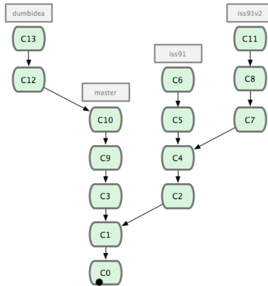
Figure 3.20: Your commit history with multiple topic branches.
