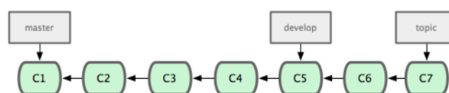
Figure 3.18: More stable branches are generally farther down the commit history.
