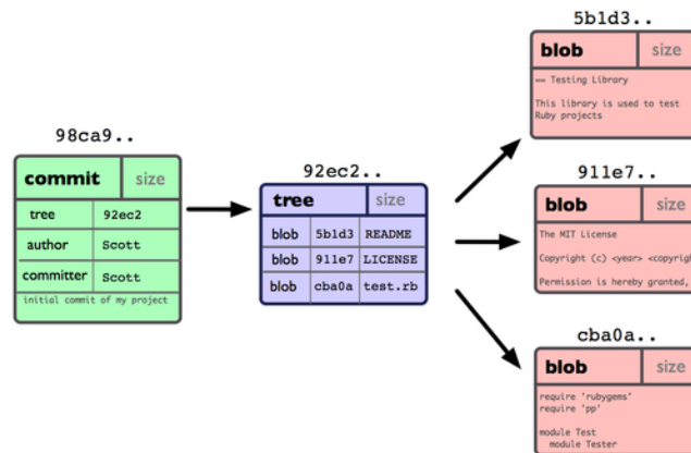
Figure 3.1: Single commit repository data.
