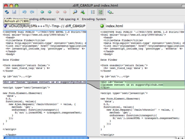
Figure 7.1: P4Merge.
