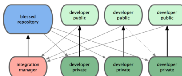
Figure 5.2: Integration-manager workflow.
