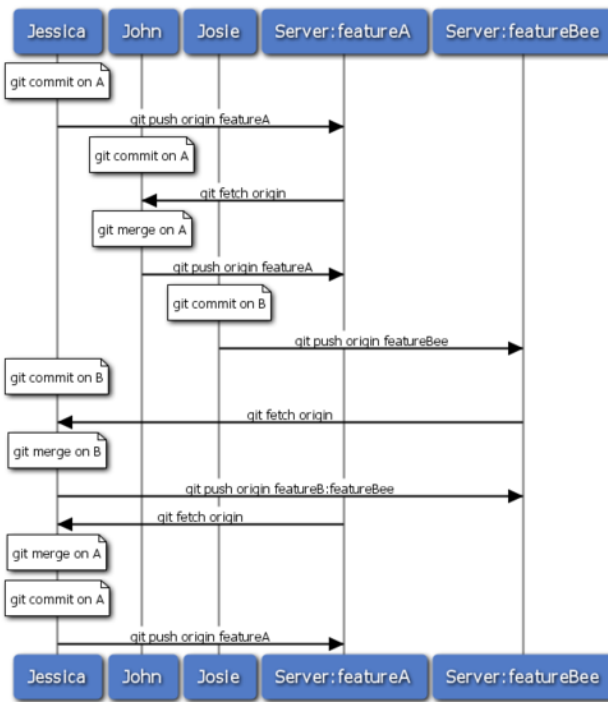
Figure 5.15: Basic sequence of this managed-team workflow.
